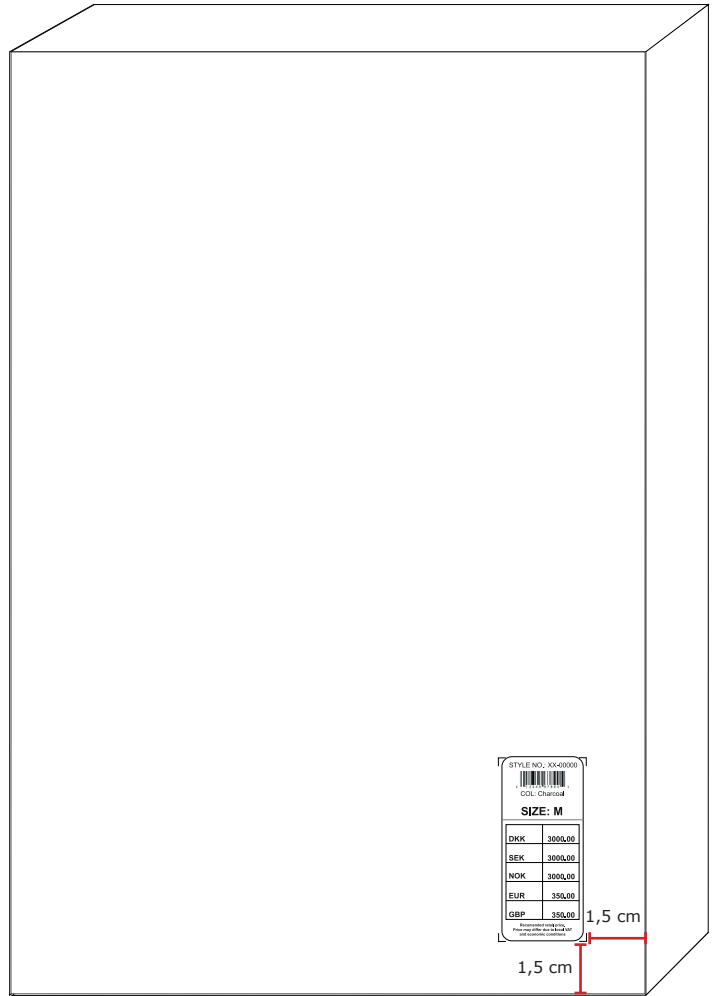
Pricesticker placement
