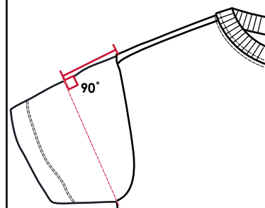
Sleeve head height
