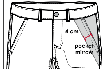
Pocket mirror with 4 cm overlap
