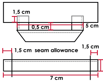
Neck strap width
